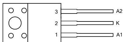
TO-220F-3 (Option 1)
